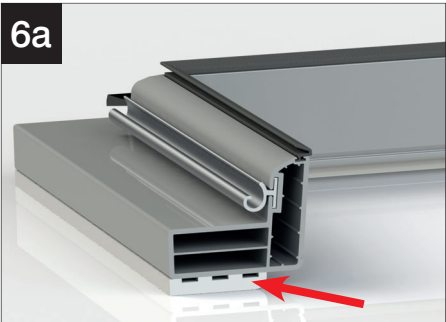
If existing glazing is 32/35mm a packer will have been pre-fitted to the frame.
